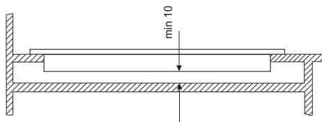
Installing hob in kitchen cabinet worktop.
