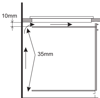
Installing hob in kitchen cabinet worktop.
